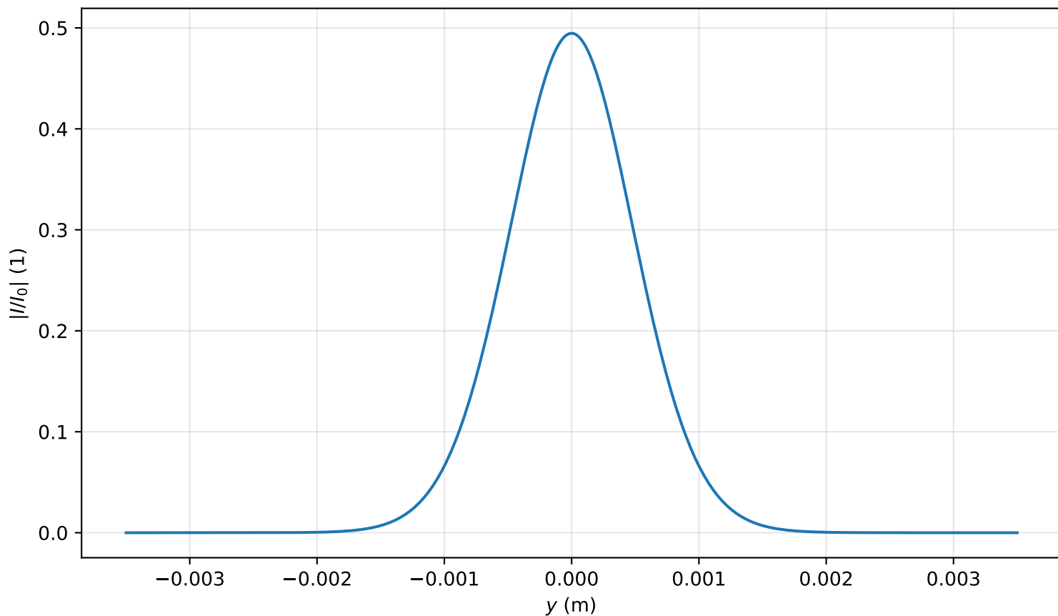
Intensity profile I(x=0, y, z=2.388)/I_0 , P_{in}=0.2P_{cr} , artificial time
